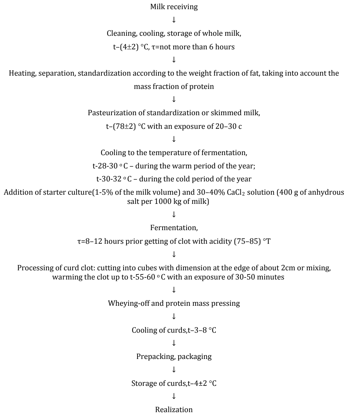
Fig. 1: Block diagram of the technological process of curds production
